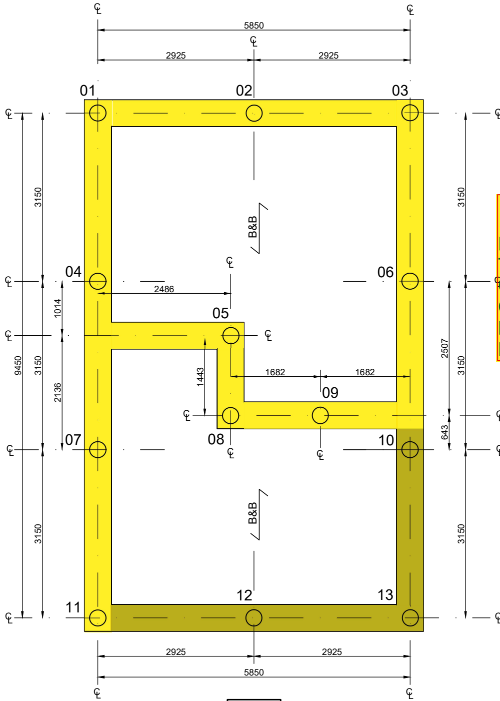
PILE AND GROUND BEAM LAYOUT PLOT 129 L363 HAM (AS)
