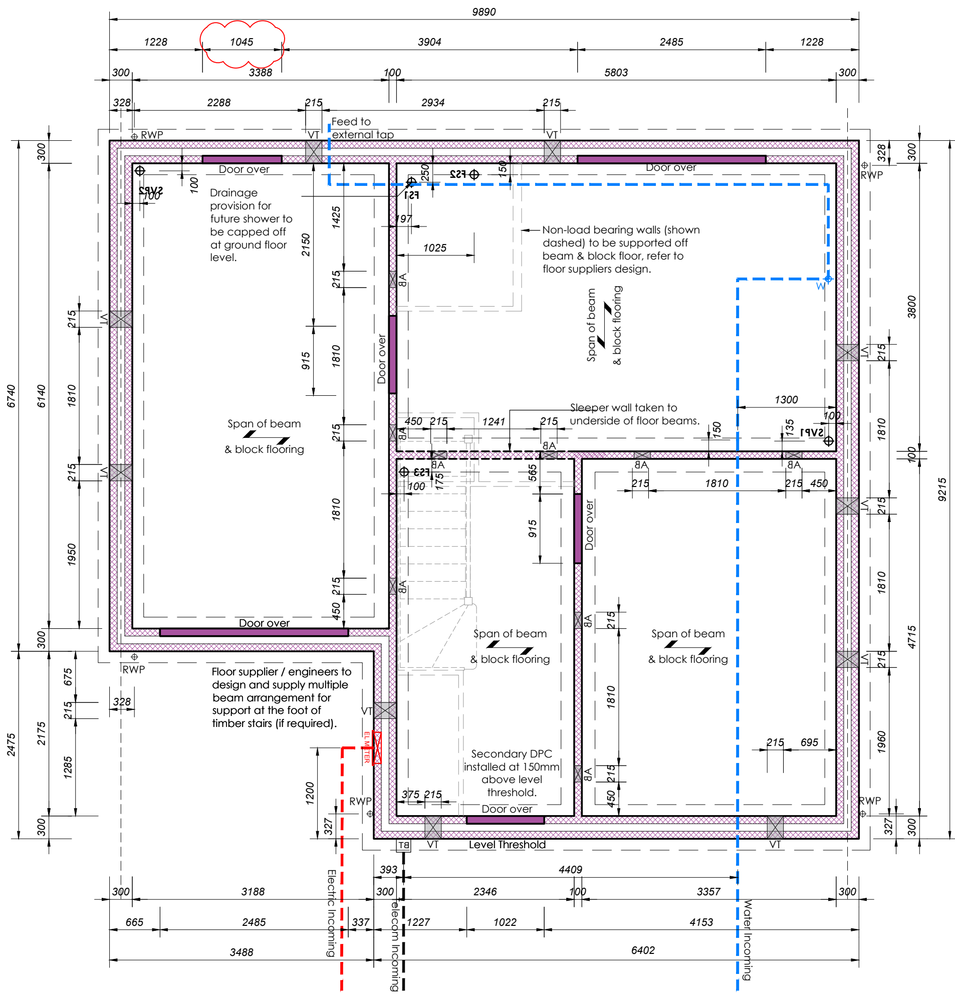
CHAWTON (CW) - SUBSTRUCTURE PLAN Scale 1:50
