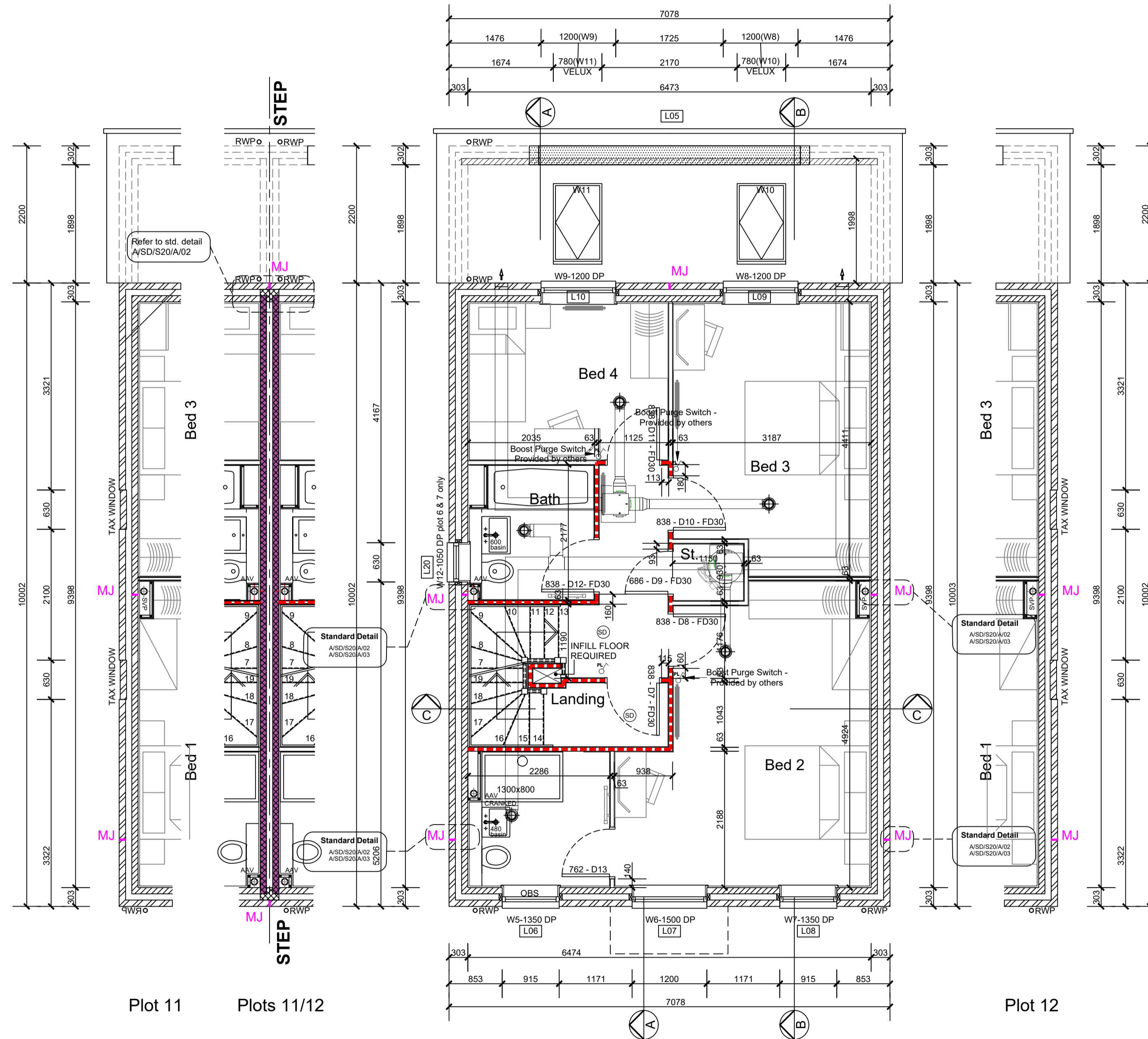
First Floor Plan Plots: 6, 7 & 12 As Plot: 11 Handed
