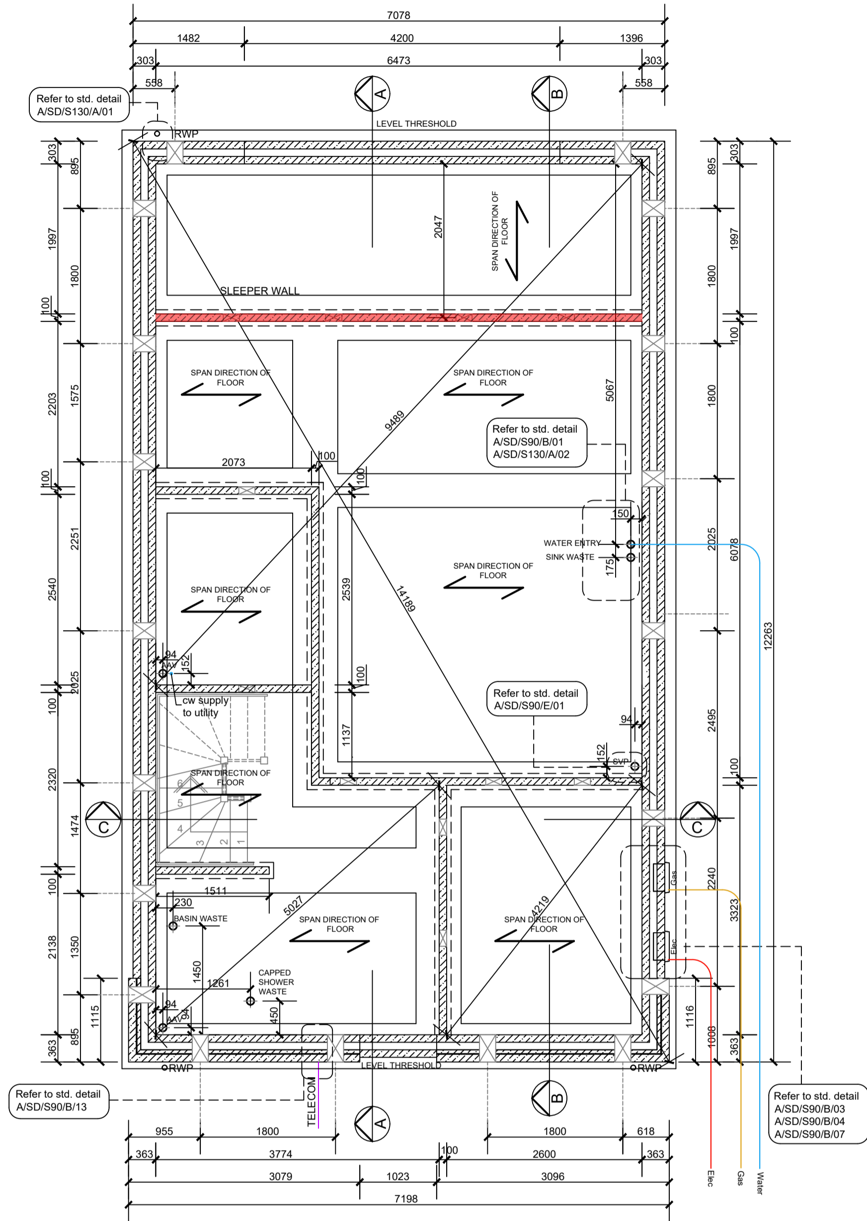
Substructure Plan Plots: 06 & 07 AS
