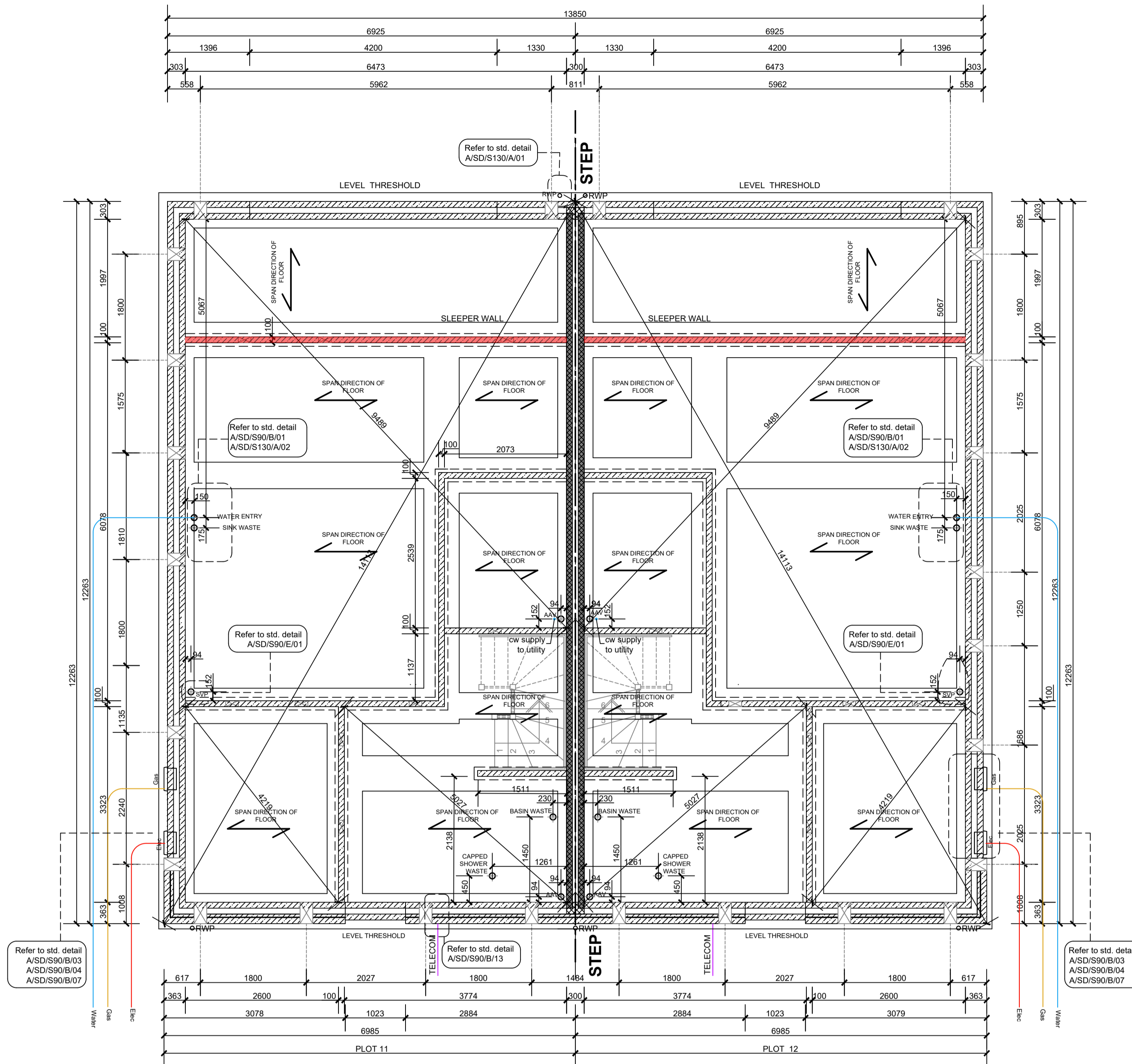
Substructure Plan Plots: 11 & 12
