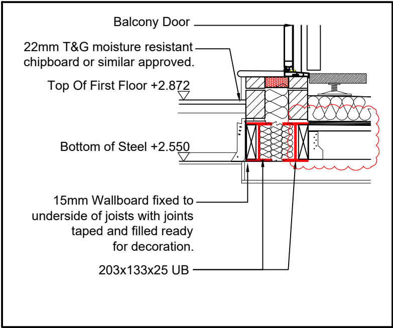
Detail B 1:20 SCALE
