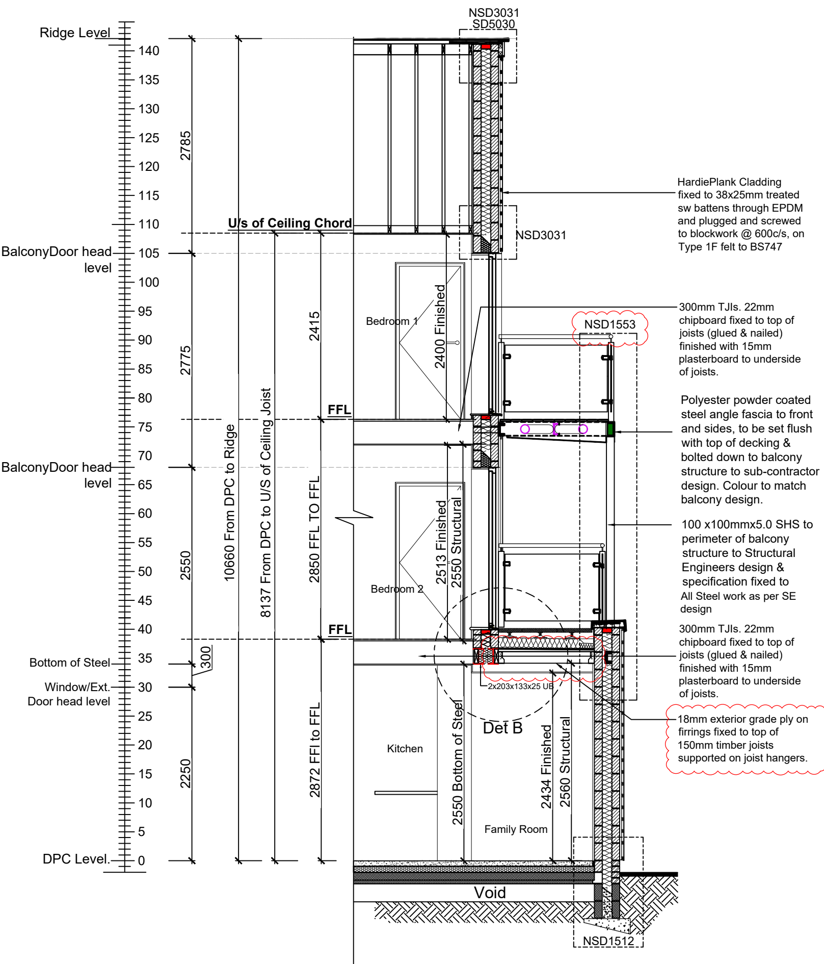
SECTION B-B 1:50 SCALE
