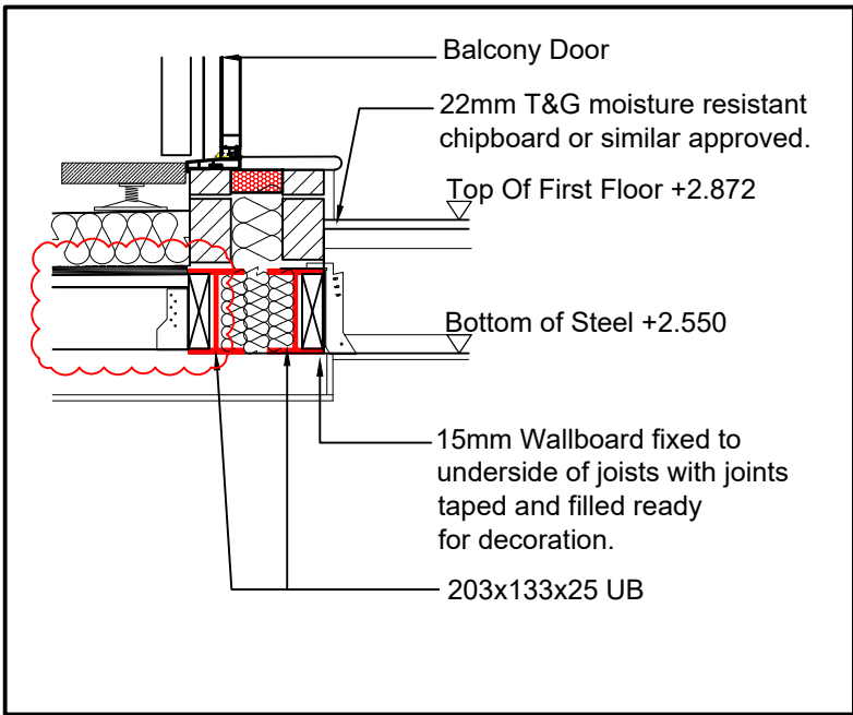
Detail B 1:20 SCALE
