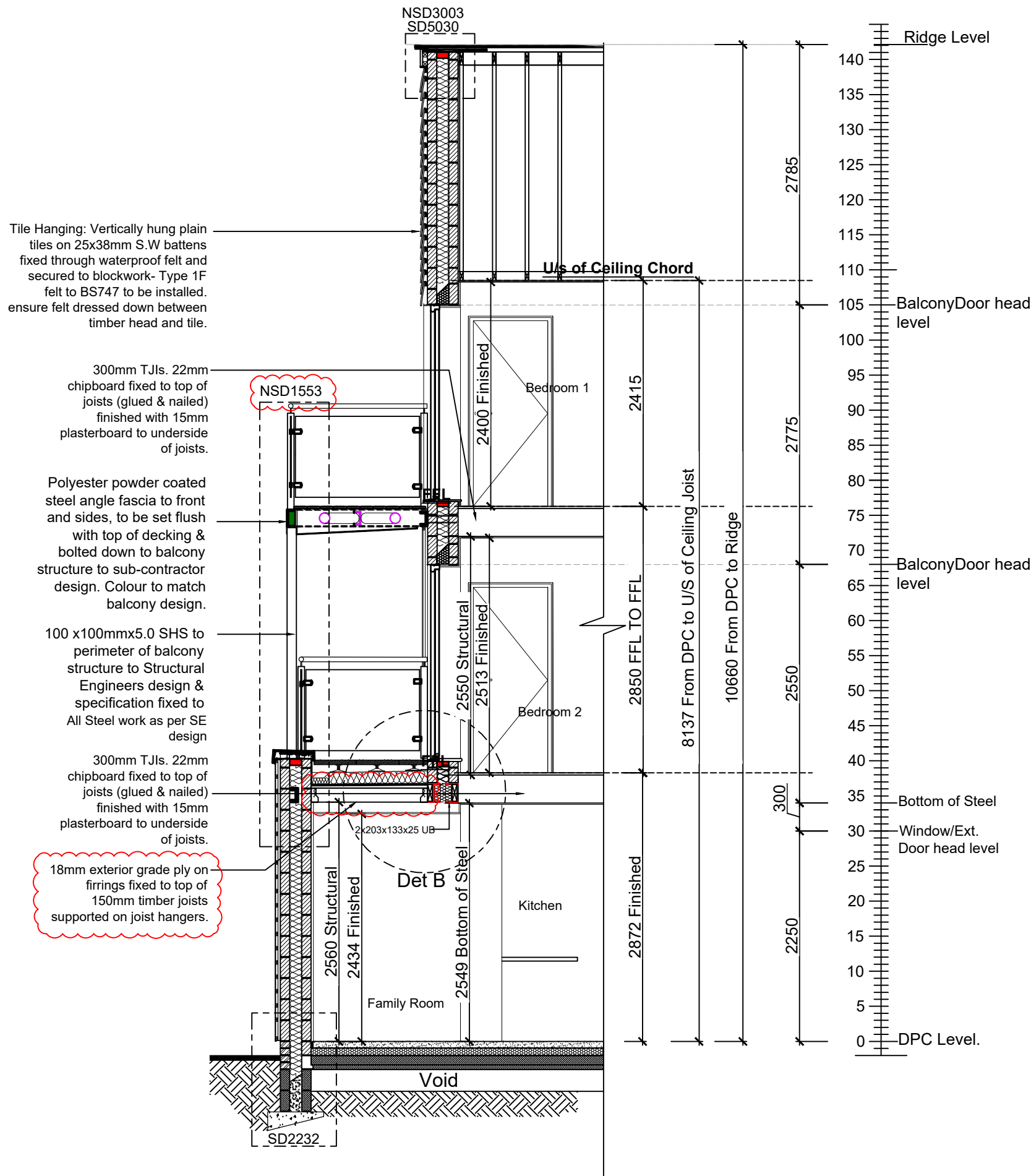
SECTION B-B 1:50 SCALE
