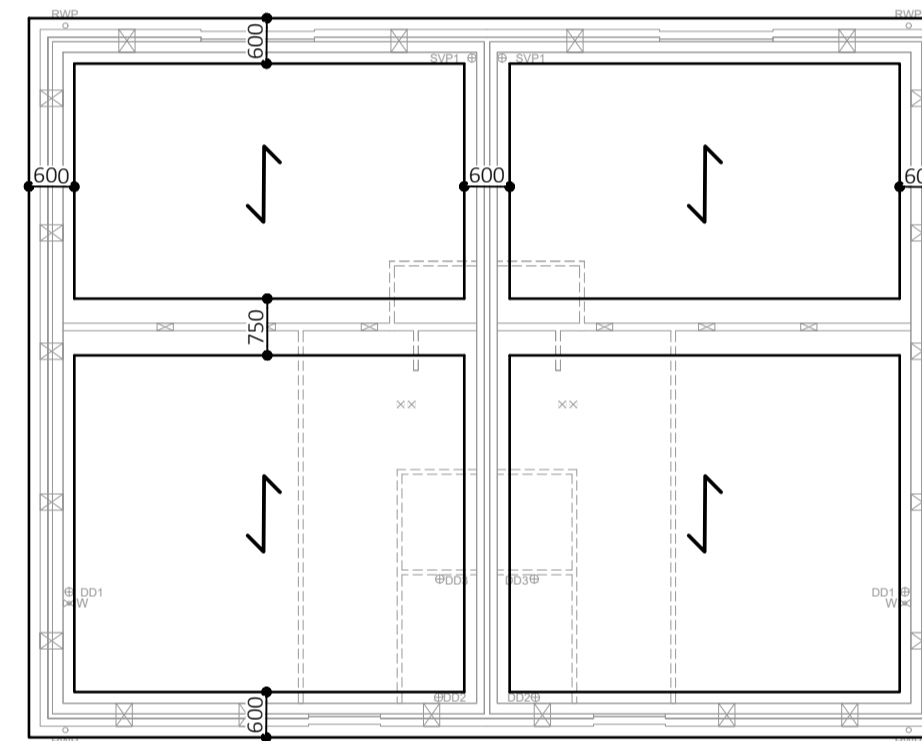
FOUNDATION LAYOUT HT CLOVER (2NO): PLOTS AS: 53, 71, 120, OPP: 52, 72, 119
