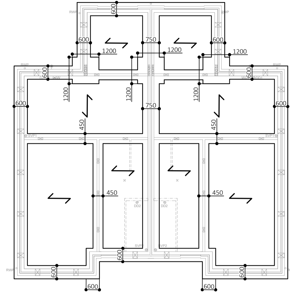
FOUNDATION LAYOUT HT FIR (2NO): PLOTS AS: 67, 69, 115, OPP: 68, 70, 114
