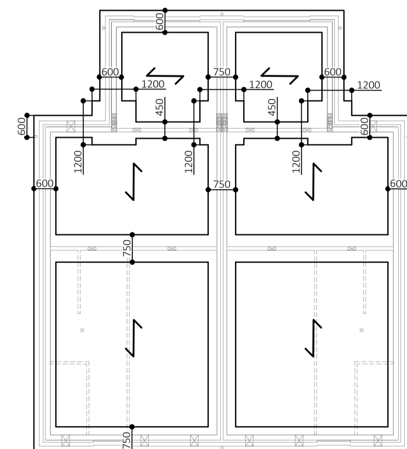
FOUNDATION LAYOUT HT ROSE (2NO) (FORMERLY FOXGLOVE 2NO): PLOTS AS: 63, 65, 74 OPP: 62, 64, 75
