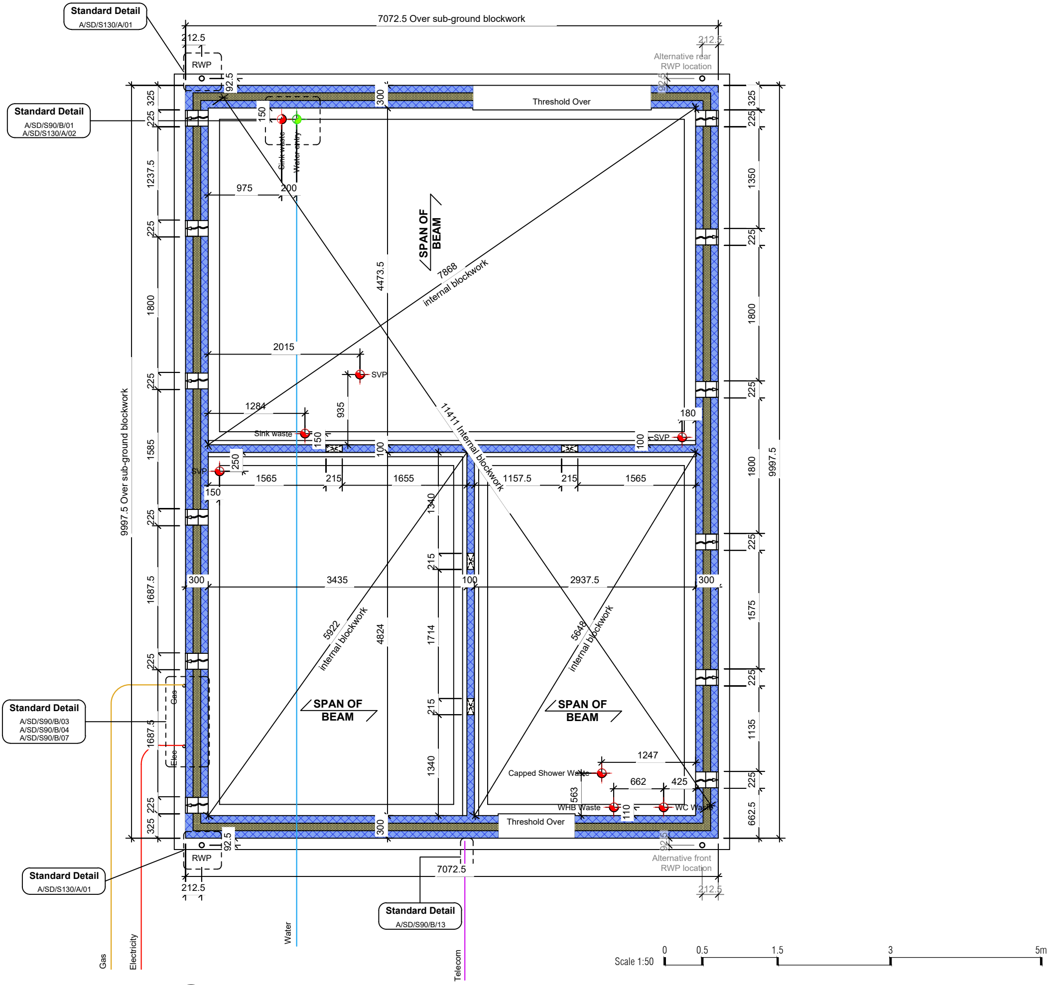
1 Foundation 1:50
