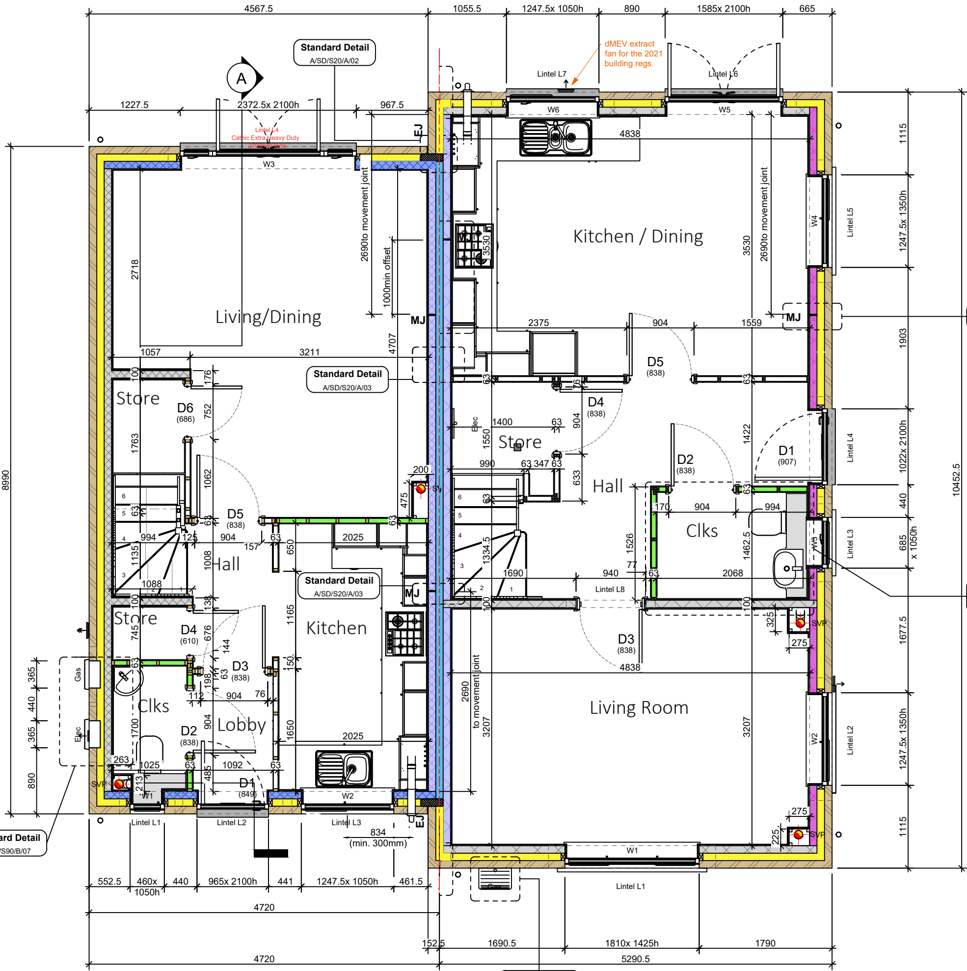
1 Block Ground Floor Plan Plots 519-520
