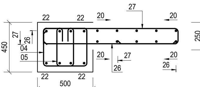
Section 3-3
