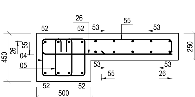
Section 5-5
