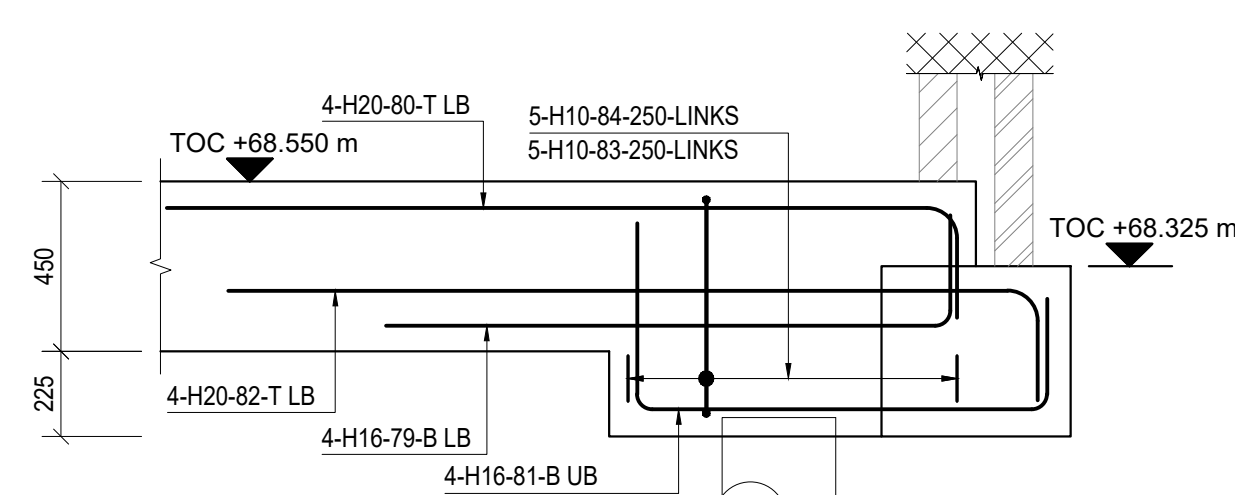
Detail-A Elevation View
