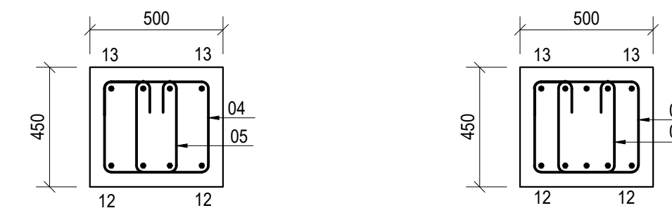
Section 1-1
