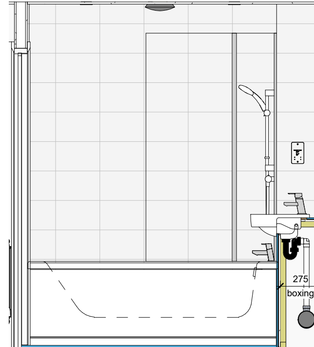
B Bathroom - View B 1 : 25
