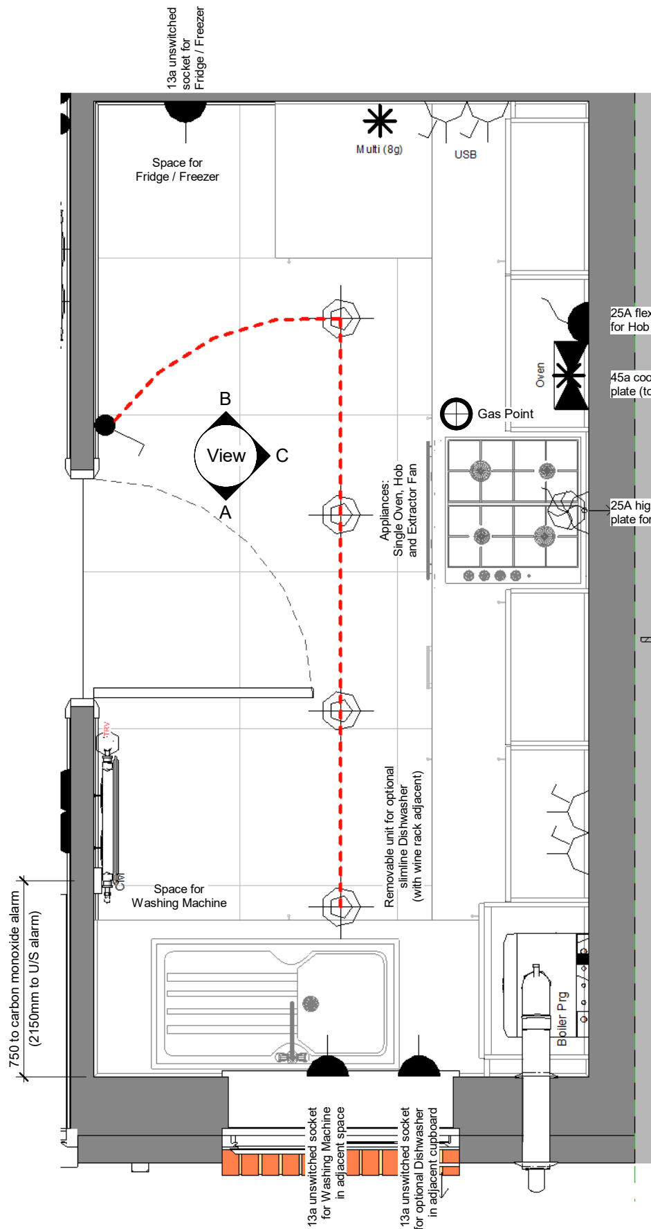
1 Kitchen Layout 1 : 20
