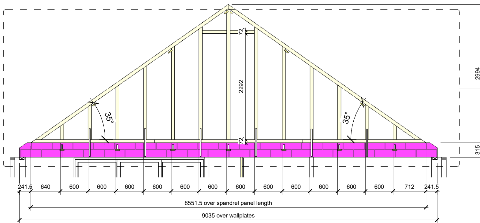
2 Spandrel Panel "SP1" (1ply, 490kg) 1 : 50
