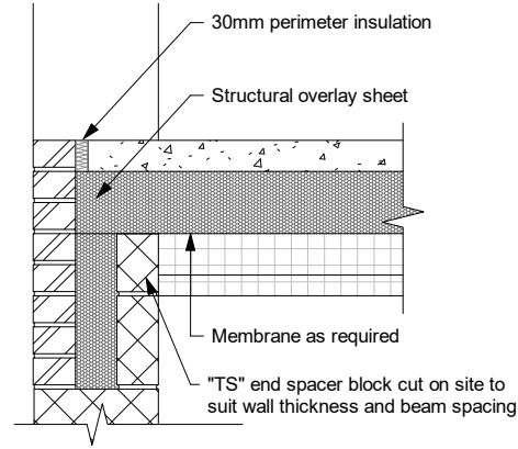
JF158 - Threshold End Detail
