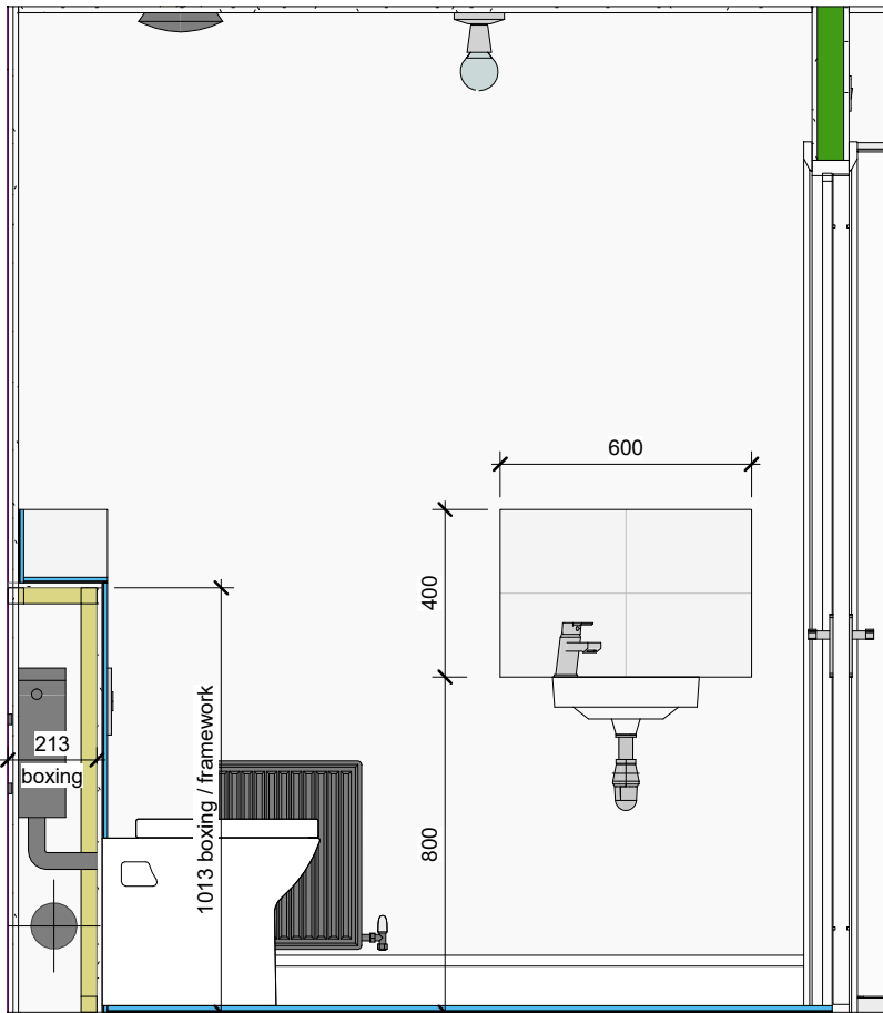
B WC - View B 1 : 20
