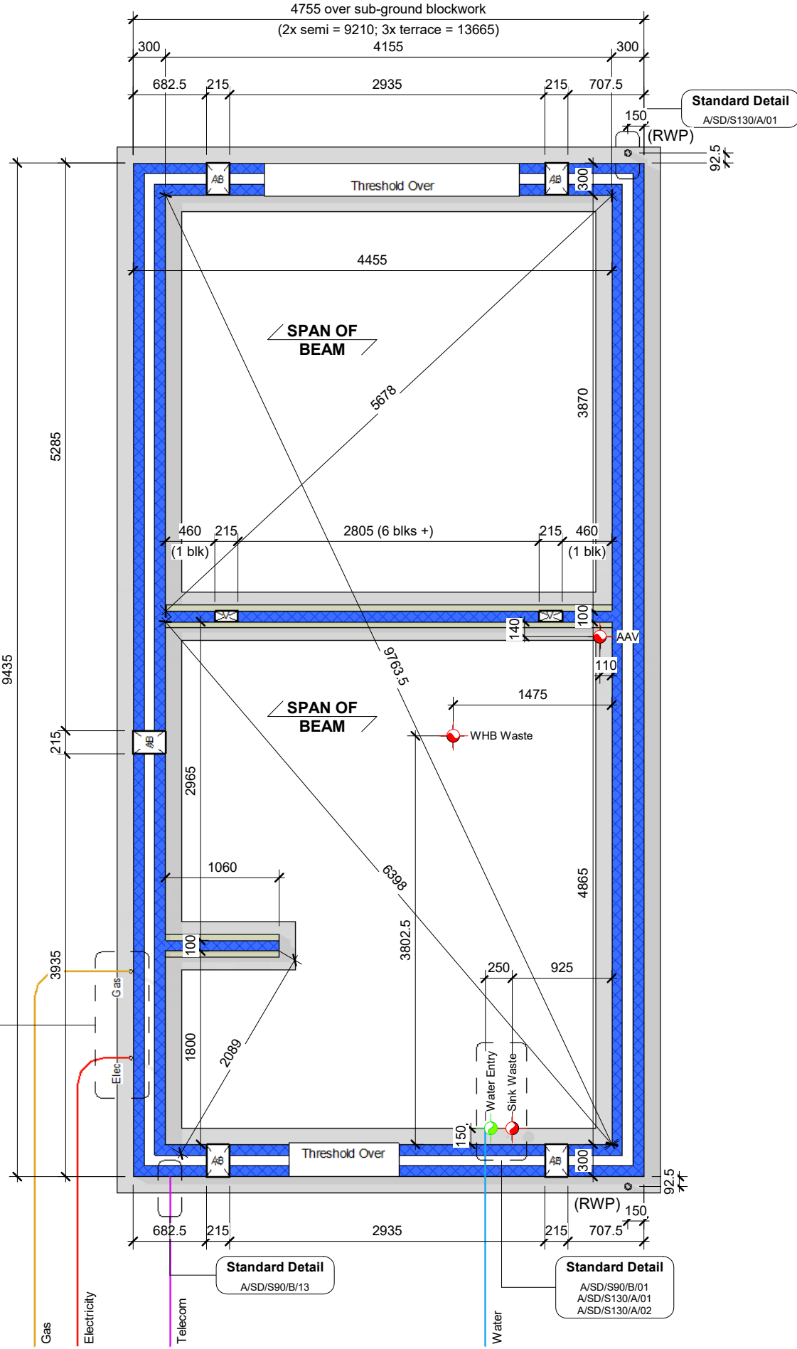
1 Foundation - Semi Detached 1 : 50
