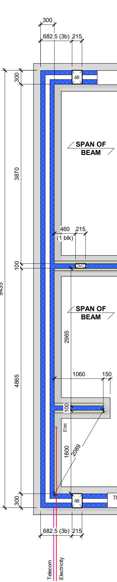
2 Foundation - Terrace Services Variation 1 : 50
