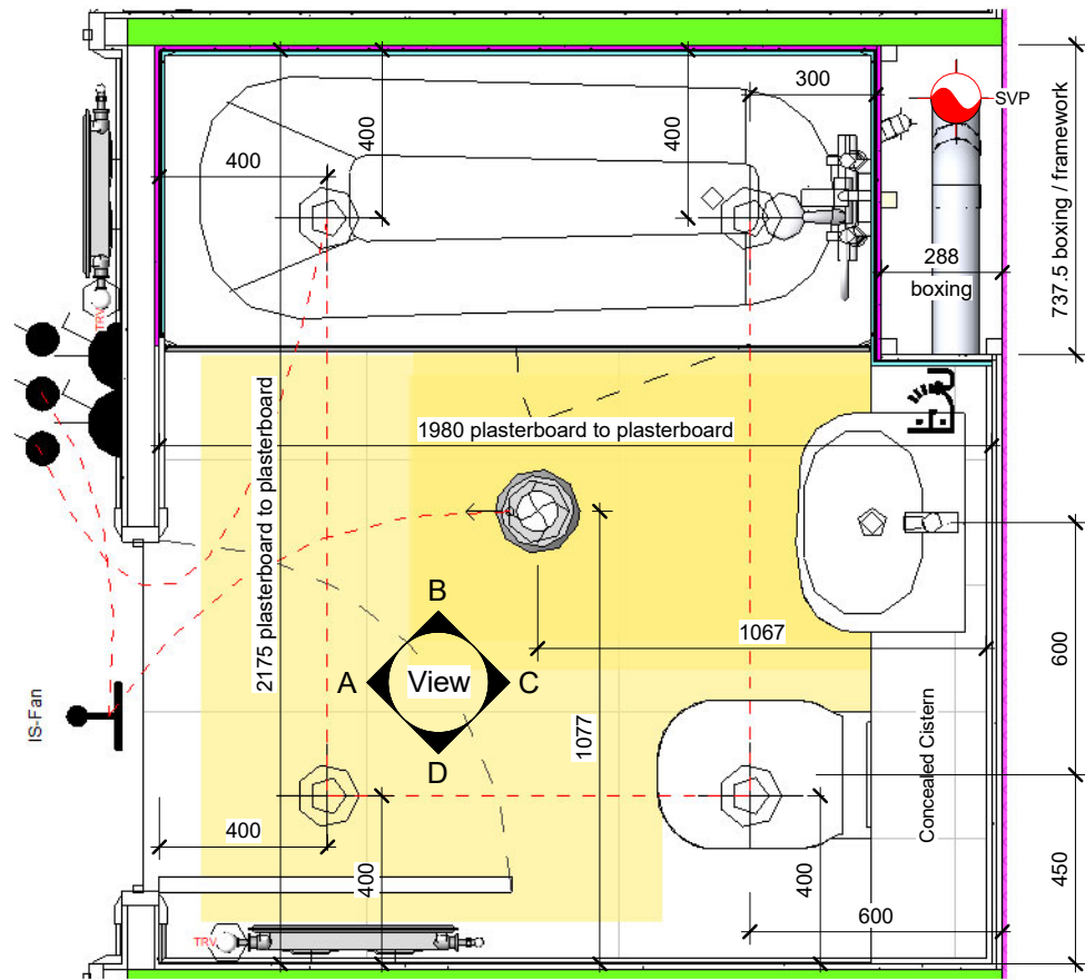
1 Bathroom Layout 1 : 20
