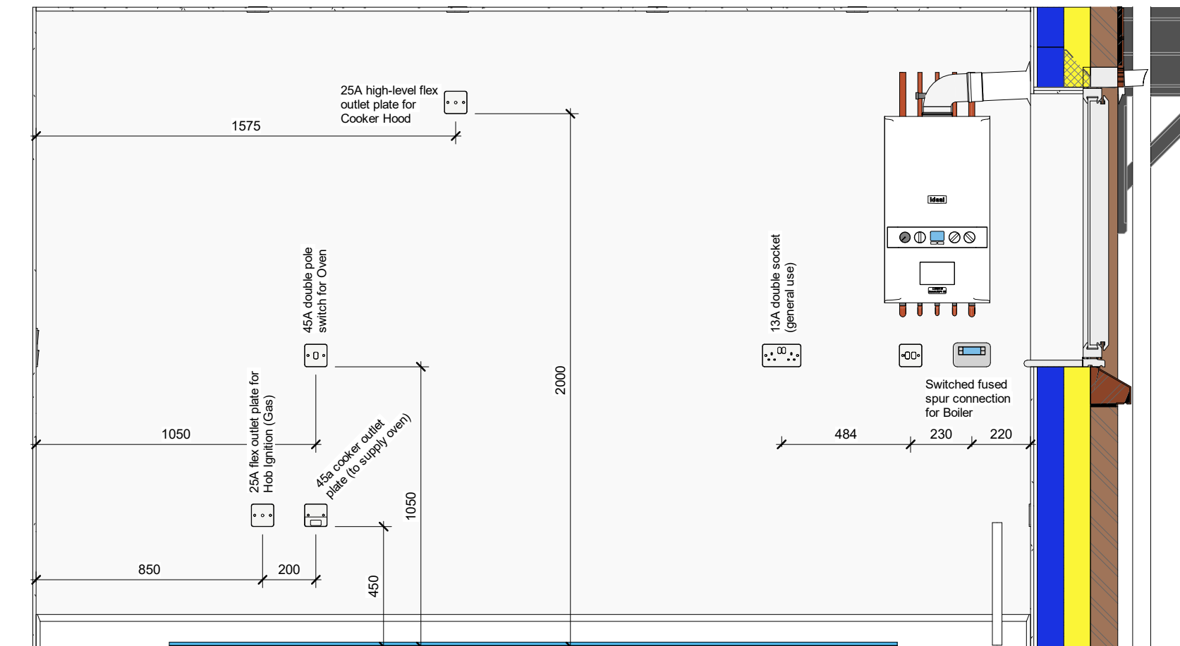
C Kitchen Electrics - View C 1 : 20
