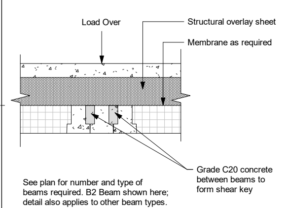
JF132 - Load Supported by Floor
