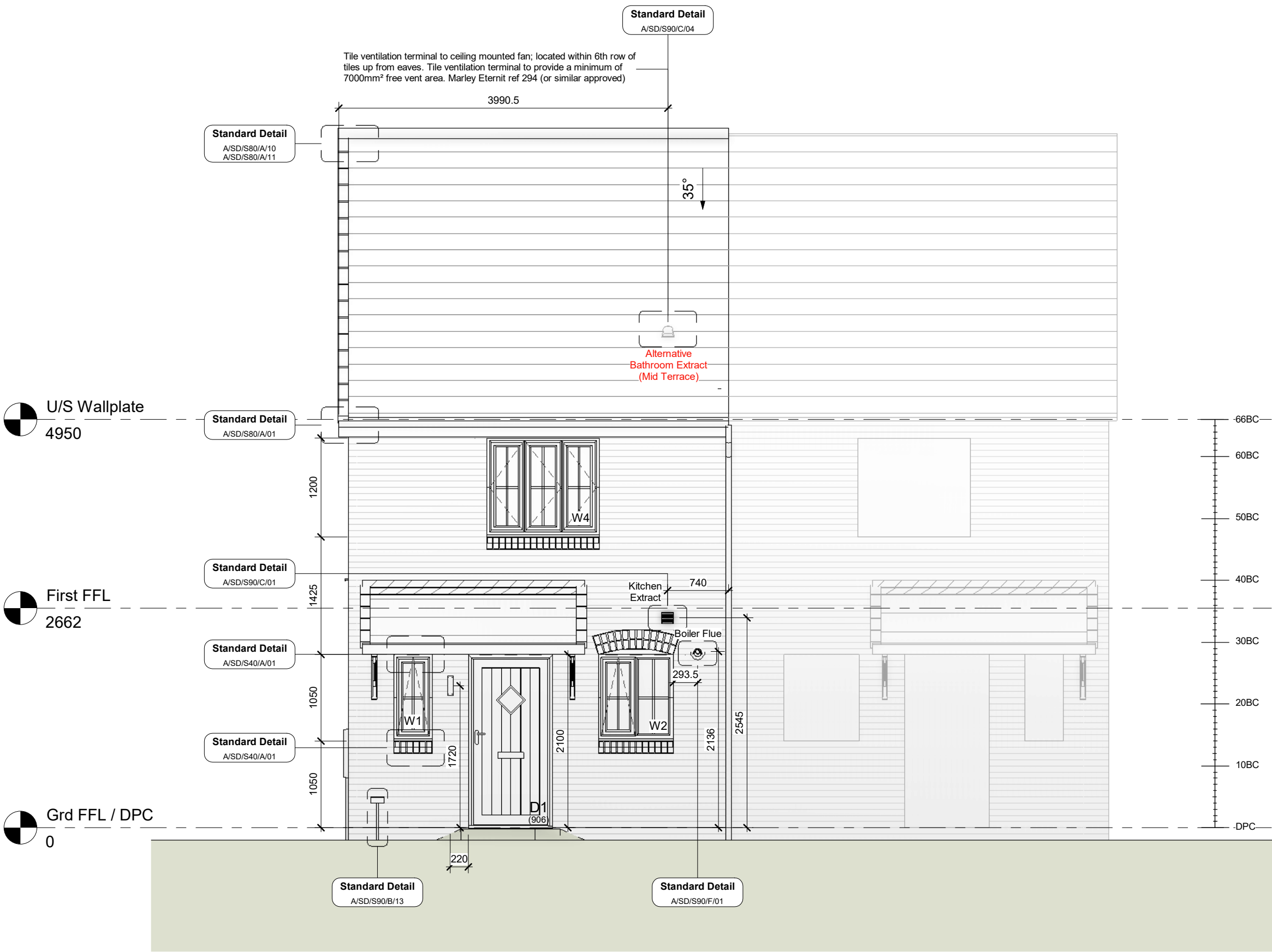
1 Front Elevation 1 : 50
