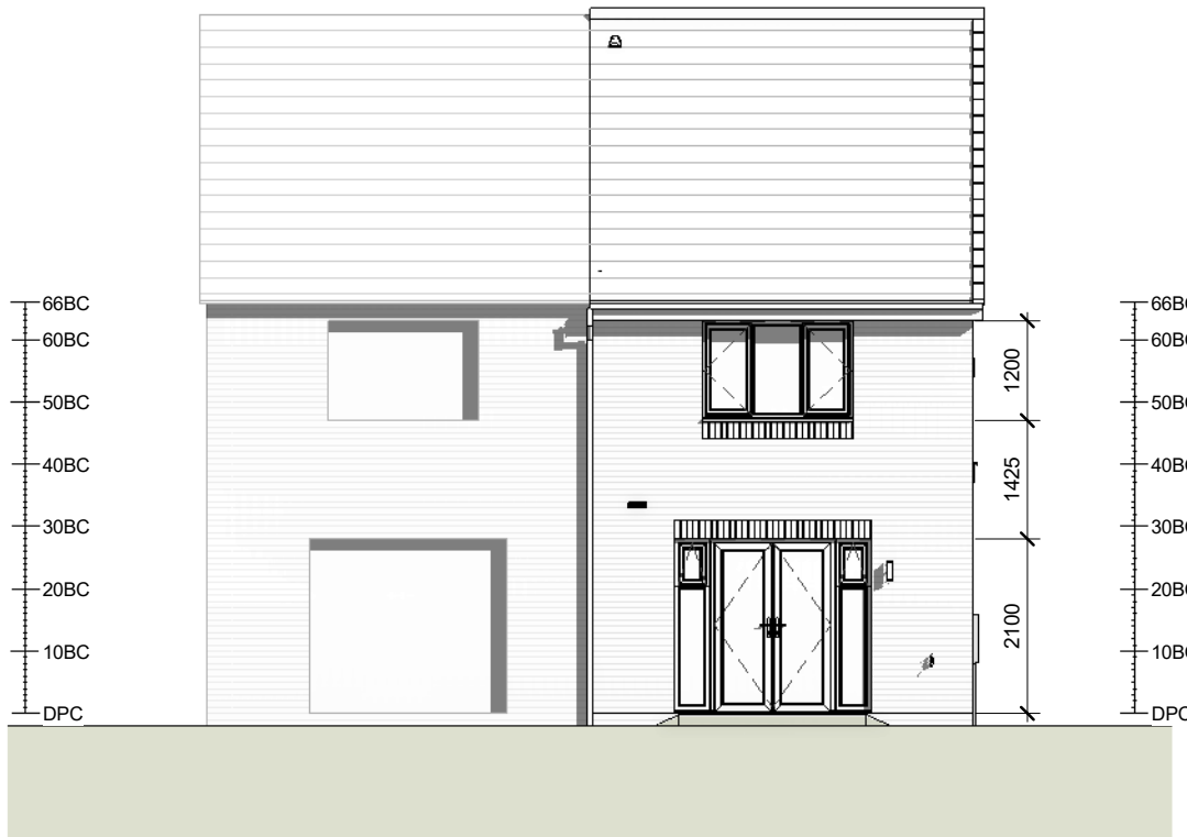
3 Rear Elevation 1 : 100
