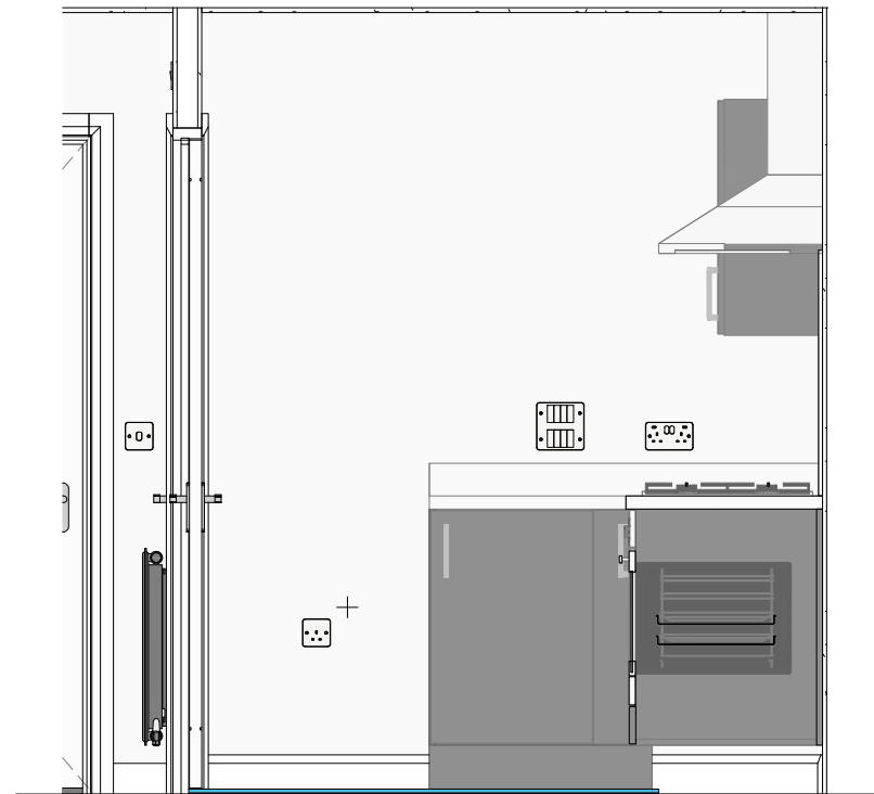
B Kitchen - View B 1 : 25
