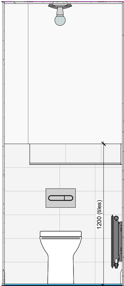
C WC - View C 1 : 20
