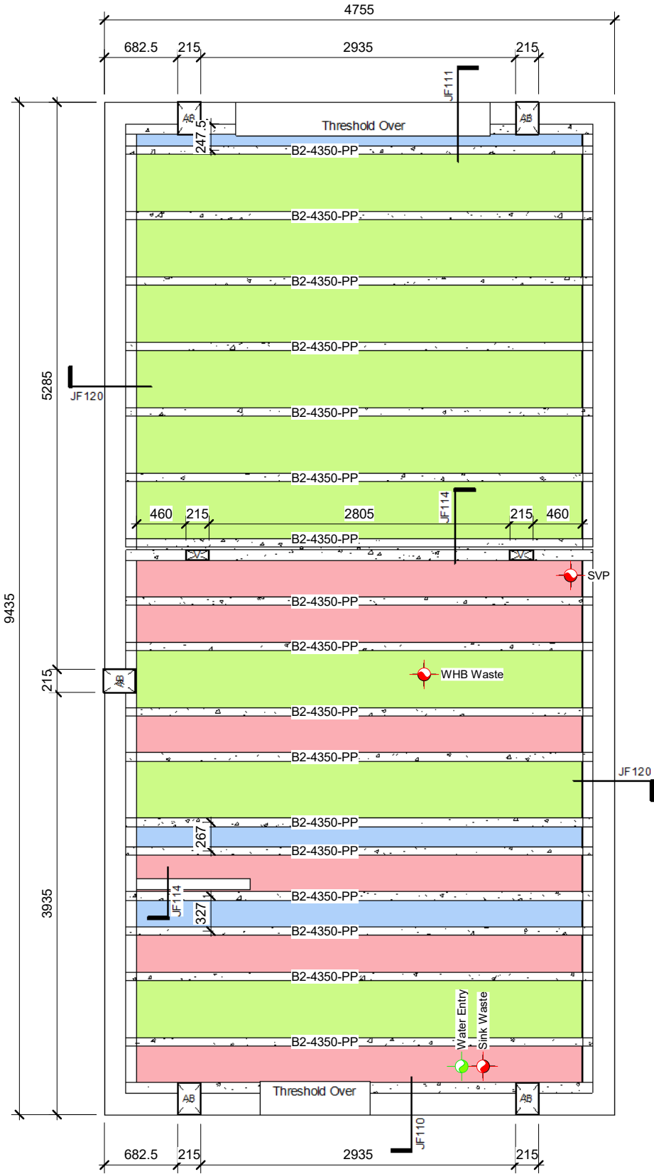
1 Beam Layout 1-50 1 : 50
