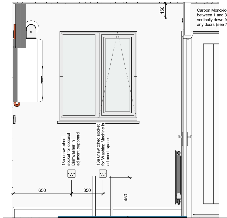
A Kitchen Electrics - View A 1 : 20
