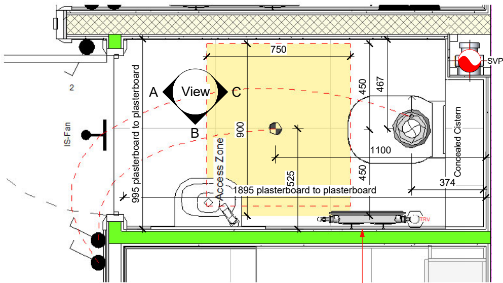
1 Ground Floor W/C Layout 1 : 20
