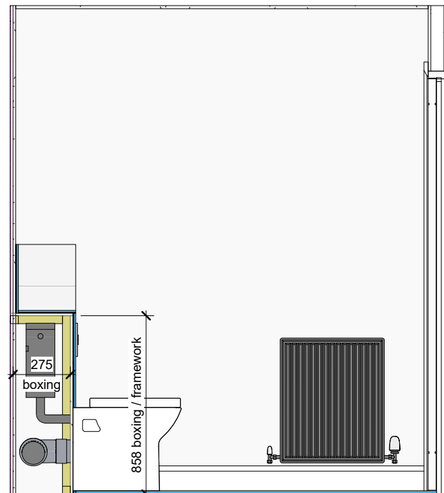
D Bathroom - View D 1 : 25
