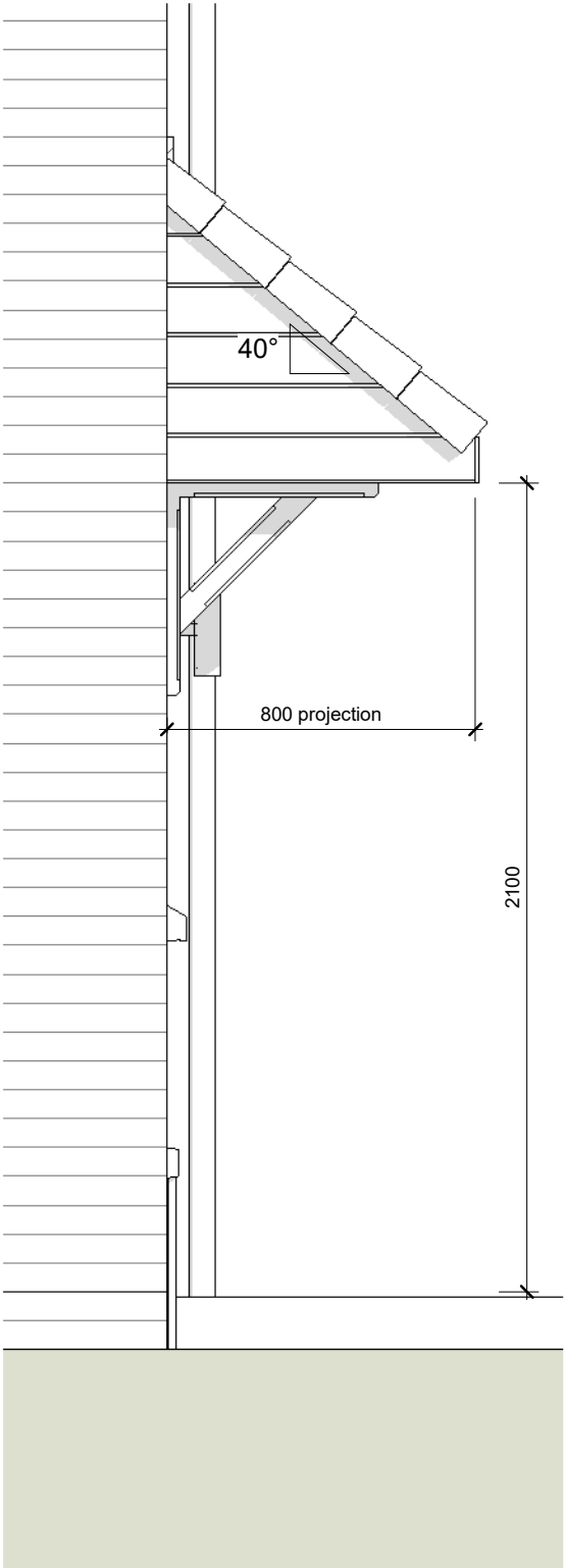
2 Gable Elevation 1 : 20
