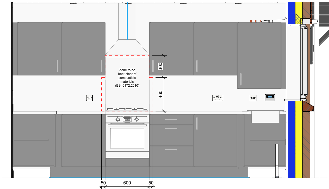
C Kitchen - View C 1 : 25
