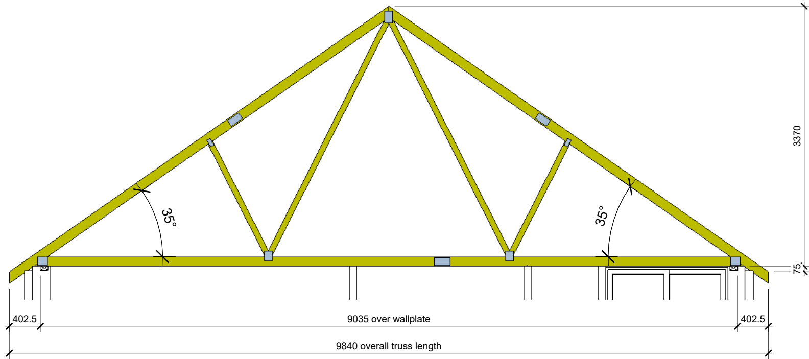
1 Truss "HP" - 8no reqd (1ply, 70kg) 1 : 50
