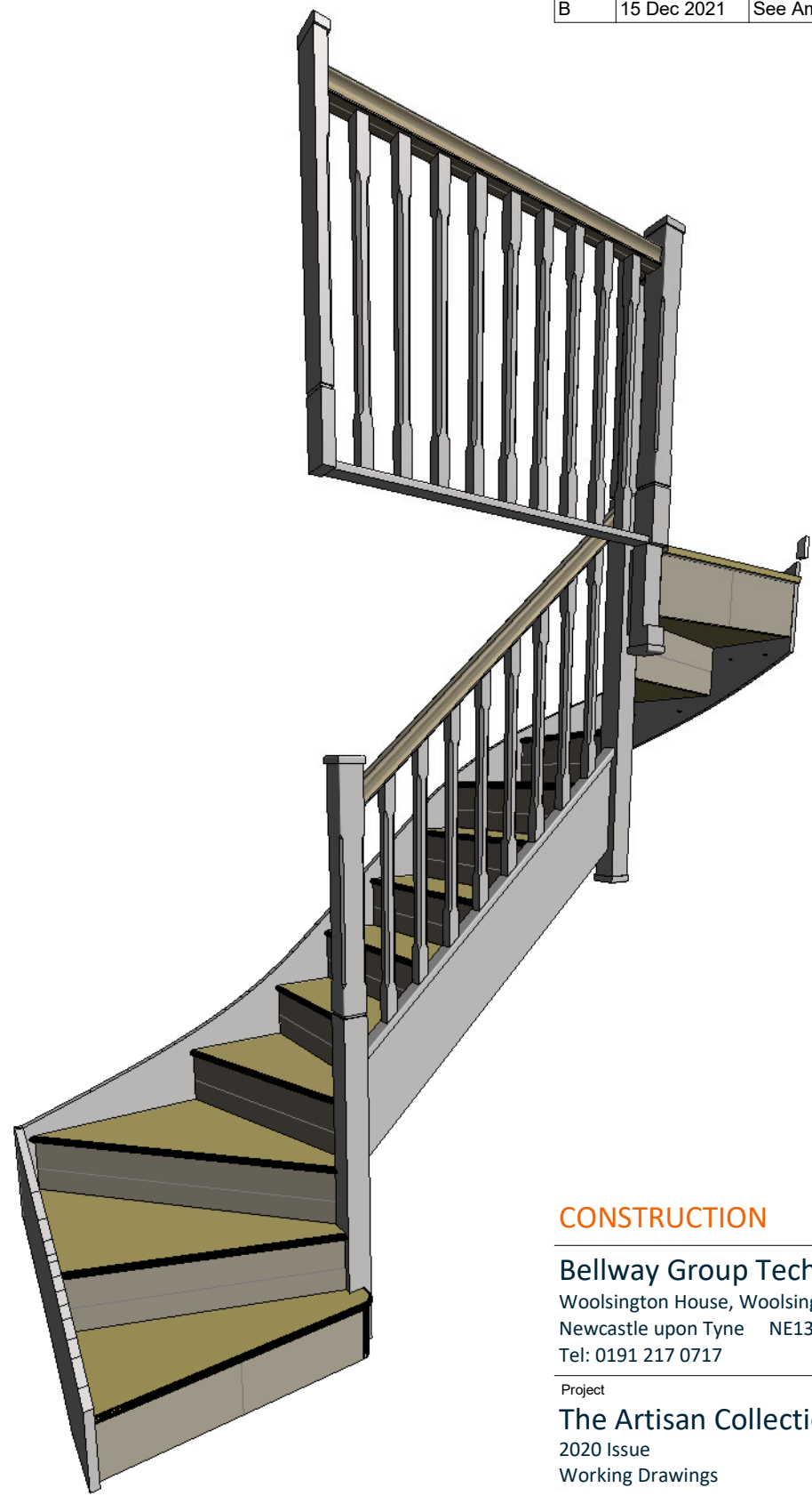
3 Staircase - 3d View
