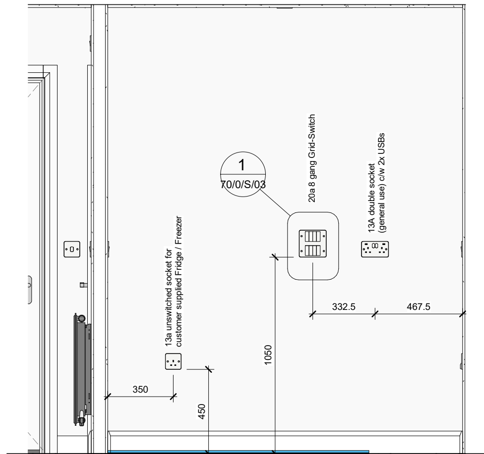
B Kitchen Electrics - View B 1 : 20
