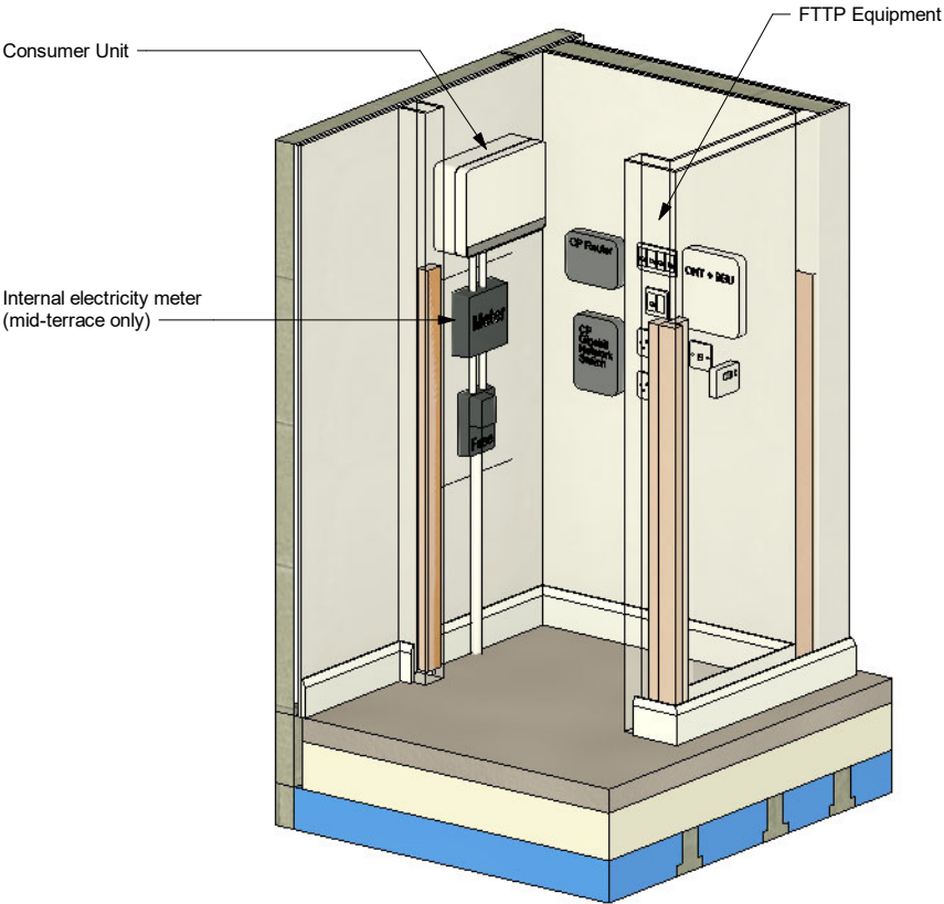
2 Mid Terrace Cup'd (View A)
