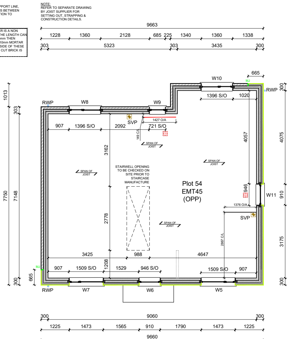
Plot 54 - First Floor Plan
