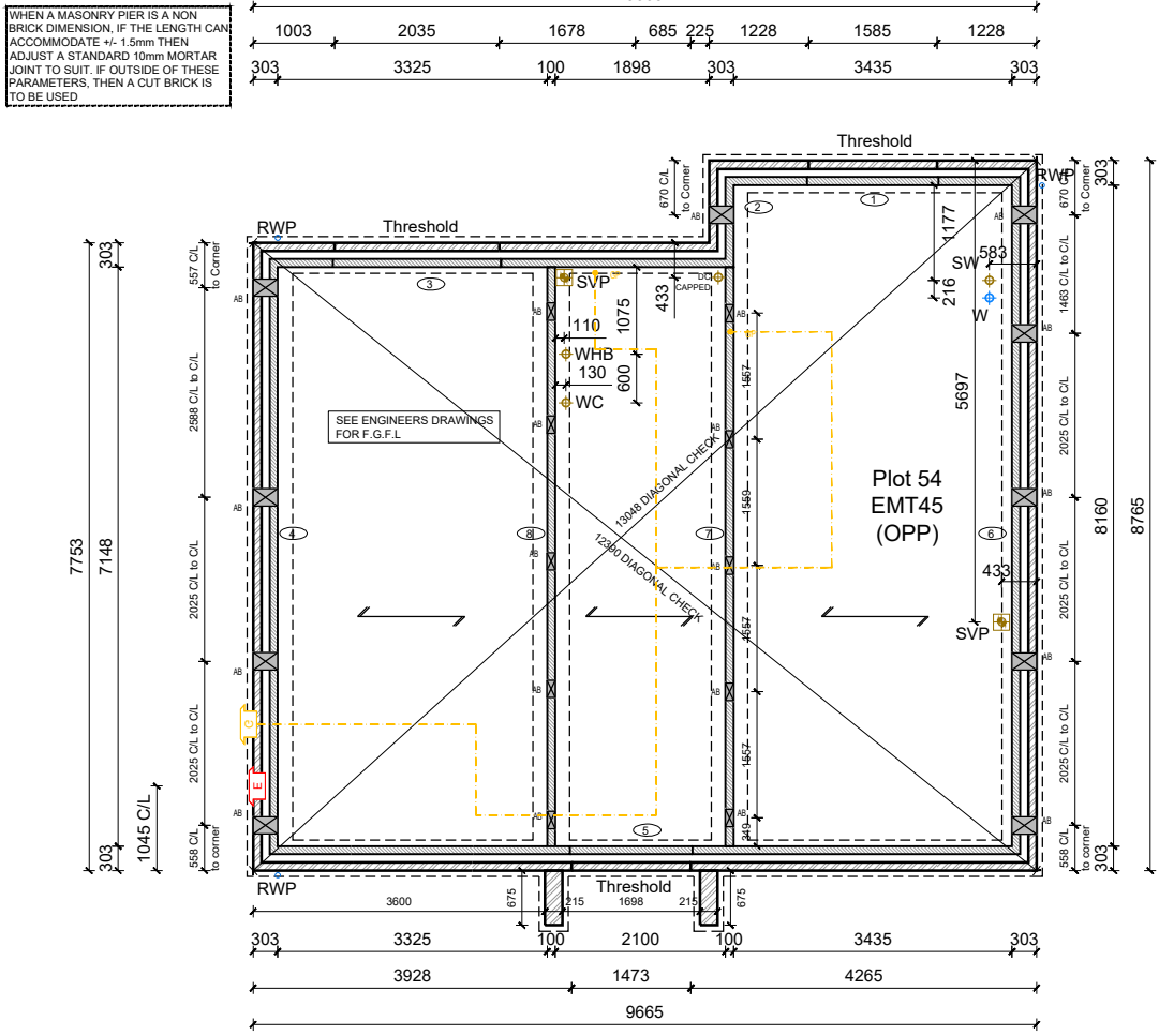
Plot 54 - Substructure Plan
