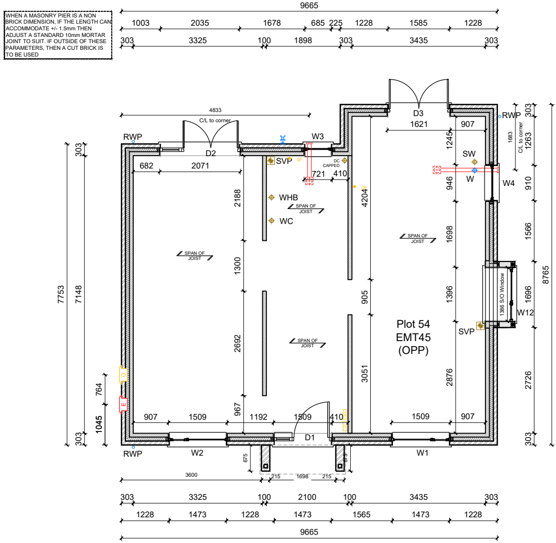
Plot 54 - Ground Floor Plan
