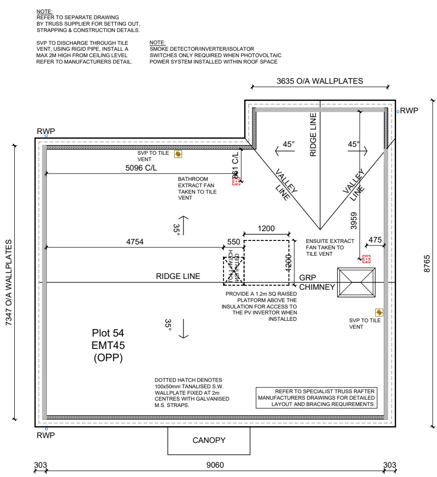
Plot 54 - Roof Plan
