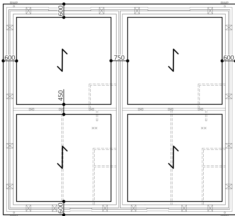
FOUNDATION LAYOUT HT BELLFLOWER (2NO): PLOTS AS: 58, 60, 99, 103, OPP: 57, 59, 98, 102
