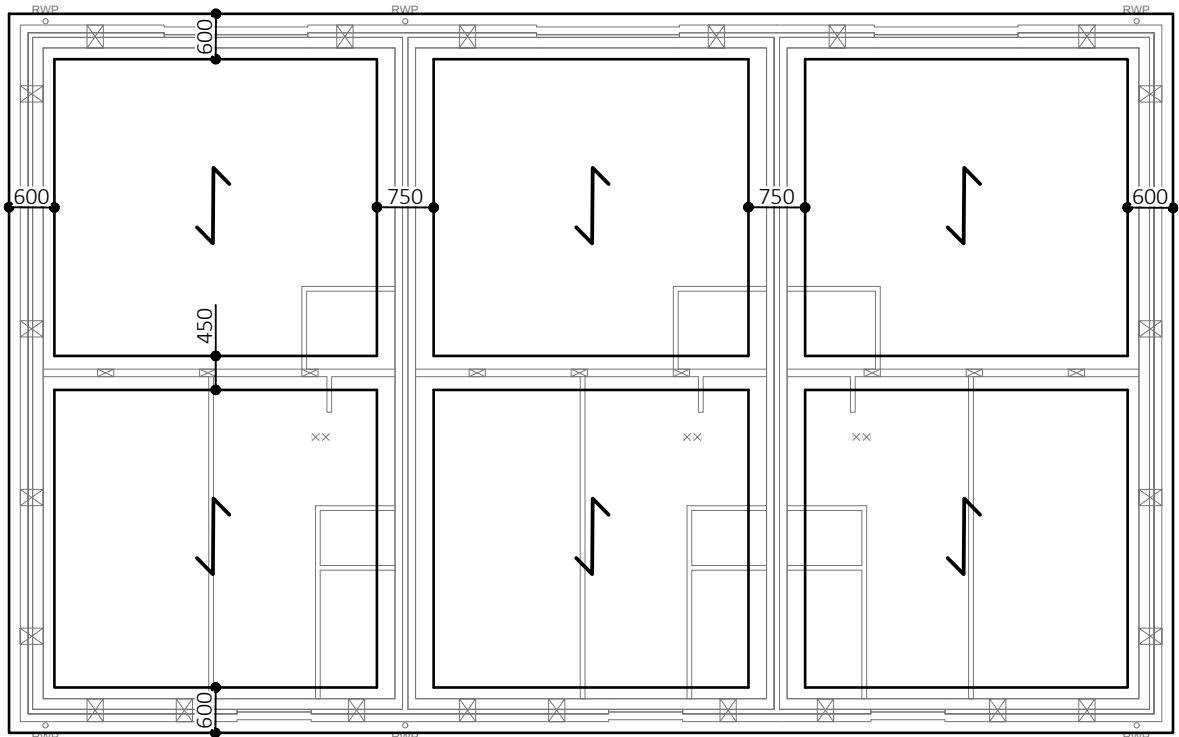
FOUNDATION LAYOUT HT BELLFLOWER (3NO): PLOTS AS: 24, 25, 45, 46, OPP: 23, 44
