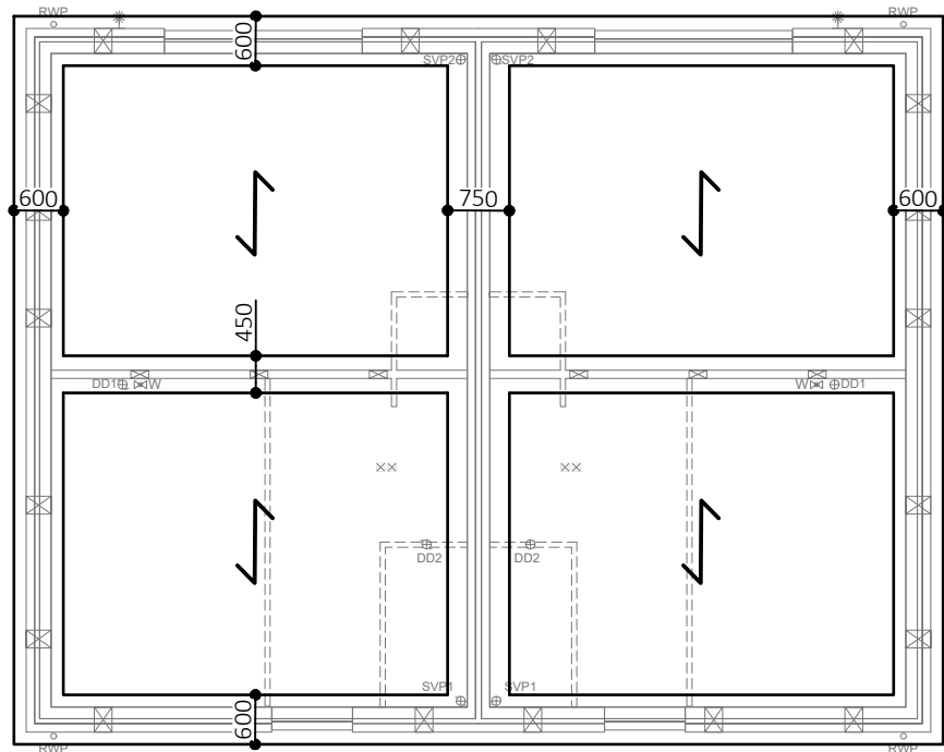
FOUNDATION LAYOUT HT BAYBERRY (2NO): PLOTS AS: 14, 22, 33, 101, OPP: 15, 21, 32, 100
