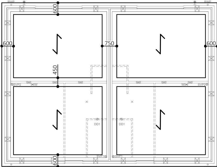
FOUNDATION LAYOUT HT ASPEN (2NO): PLOTS AS: 56, OPP: 55
