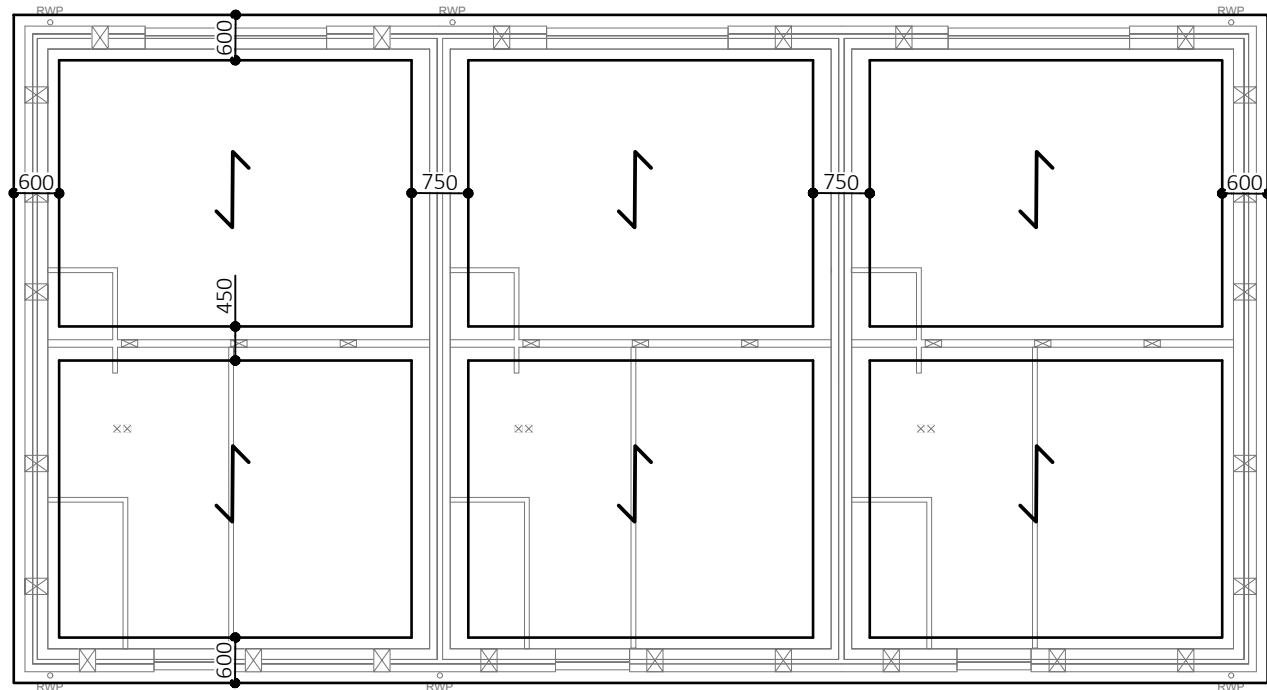
FOUNDATION LAYOUT HT BAYBERRY (3NO): PLOTS AS: 49, OPP: 16, 17, 18, 47, 48
