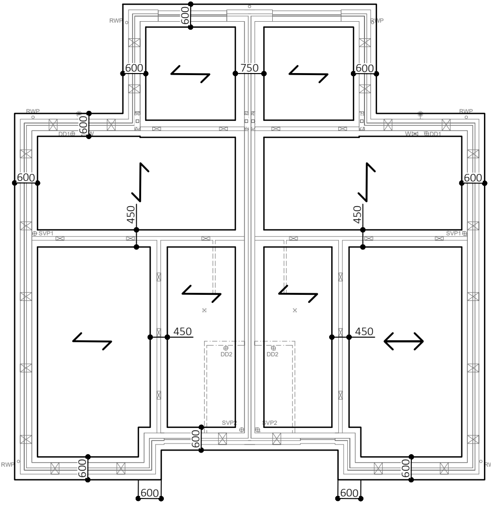
FOUNDATION LAYOUT HT FIR (2NO): PLOTS AS: 67, 69, 115, OPP: 68, 70, 114
