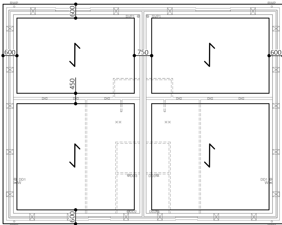
FOUNDATION LAYOUT HT CLOVER (2NO): PLOTS AS: 53, 71, 120, OPP: 52, 72, 119
