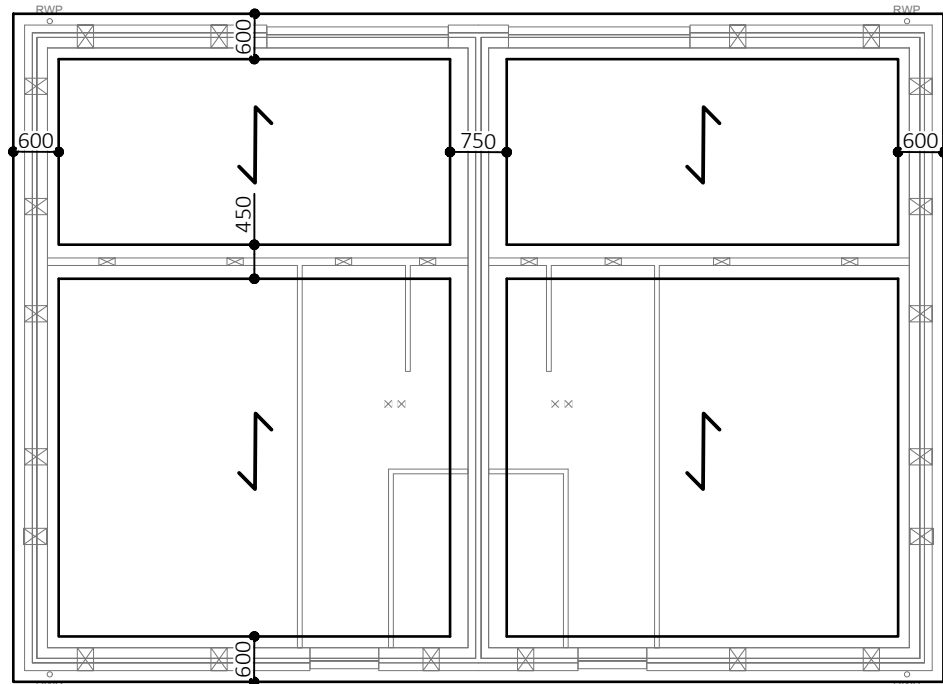
FOUNDATION LAYOUT HT BLACKTHORN (2NO): PLOTS AS: 19, OPP: 20
