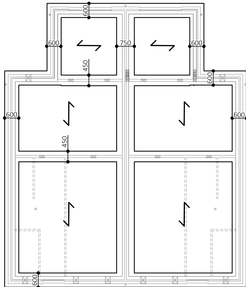
FOUNDATION LAYOUT HT FOXGLOVE (2NO): PLOTS AS: 63, 65, 74 OPP: 62, 64, 75
