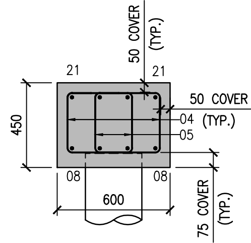
SECTION 1-1 SCALE 1:20
