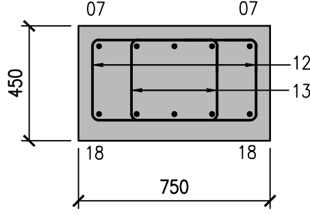
SECTION 3-3 SCALE 1:20
