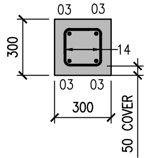
SECTION 2-2 SCALE 1:20
