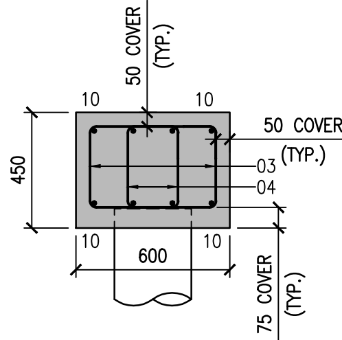
SECTION 1-1
