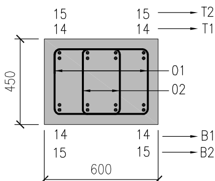
SECTION 3-3
