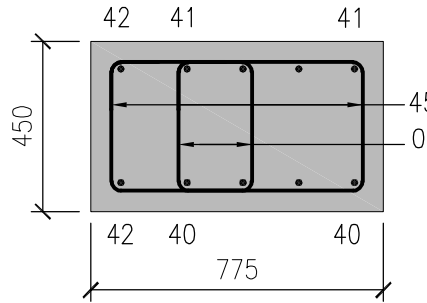
SECTION 5-5
