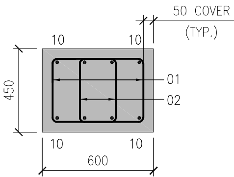
SECTION 1-1
