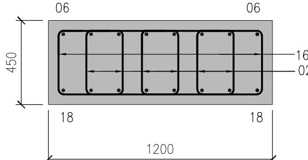
SECTION 4-4
