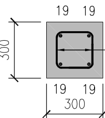
SECTION 2-2
