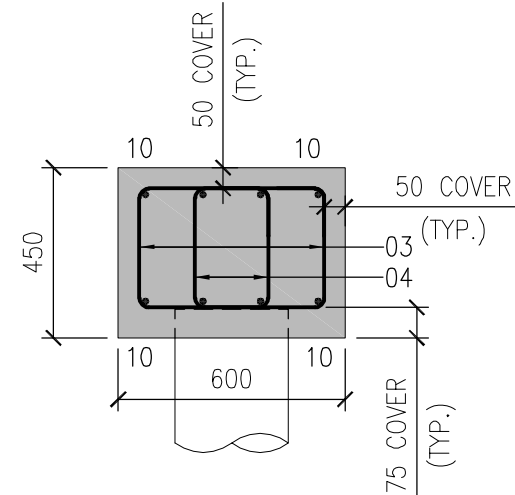
SECTION 1-1
